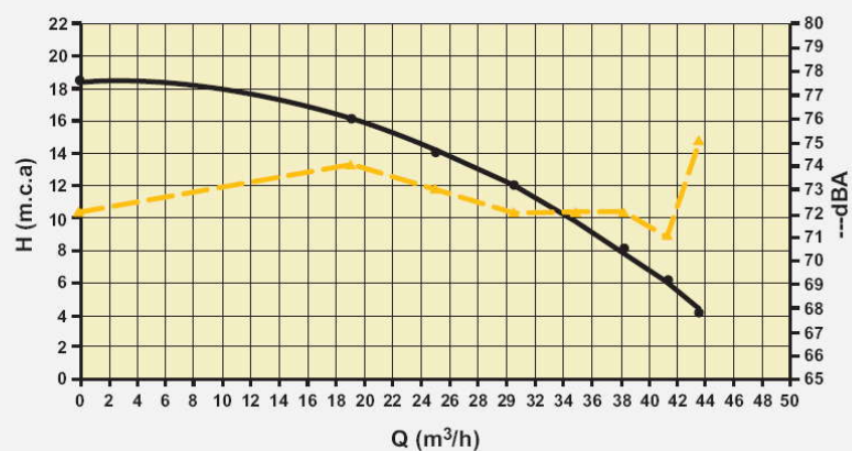
BOMBA "TRENT" 3 Cv. / "TRENT" PUMP 3 Hp
