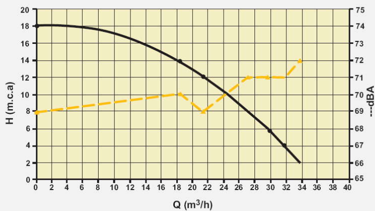
BOMBA "TRENT" 2 Cv. / "TRENT" PUMP 2 Hp
