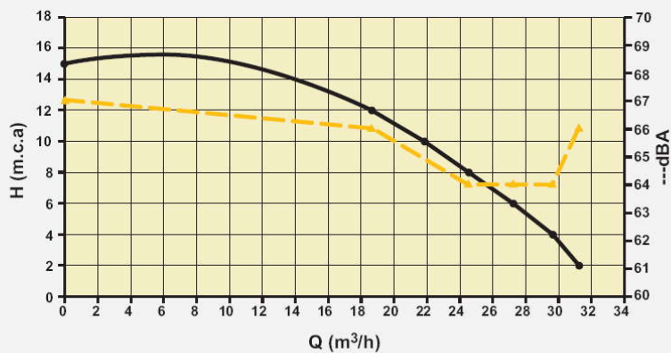
BOMBA "TRENT" 1,5 Cv. / "TRENT" PUMP 1.5 Hp
