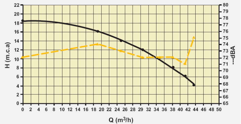
BOMBA "TRENT" 3 Cv. / "TRENT" PUMP 3 Hp
