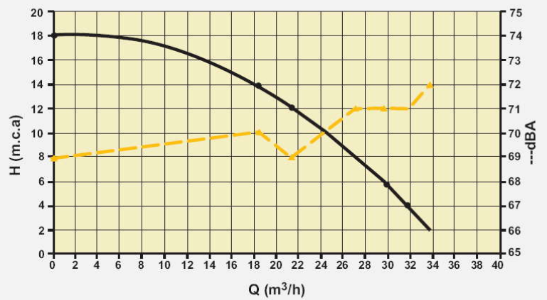
BOMBA "TRENT" 2 Cv. / "TRENT" PUMP 2 Hp
