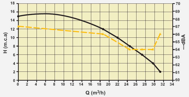
BOMBA "TRENT" 1,5 Cv. / "TRENT" PUMP 1.5 Hp
